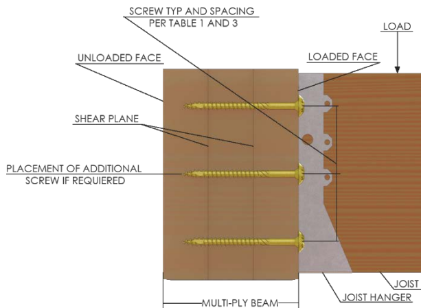
FIGURE 3. PLANE DETAIL 'A-A'
