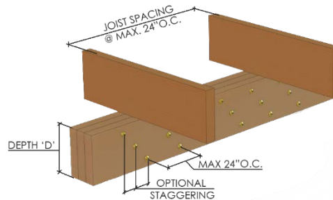
FIGURE 4. Multi-Ply Beam Top Loaded
